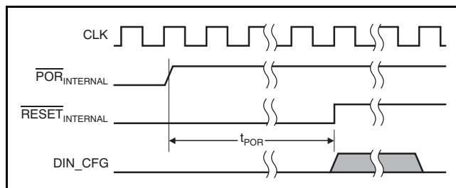
Figure 17. Power-Up Timing
