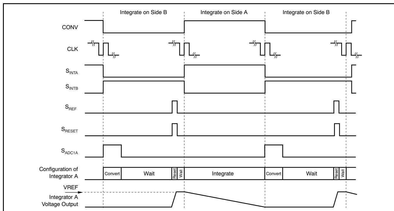
Figure 6. Conceptual Basic Integration Timing Diagram of Integrator A (as Illustrated in Figure 5)
