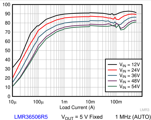
Figure 9-8. Efficiency
