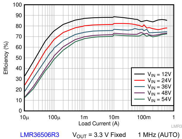
Figure 9-4. Efficiency
