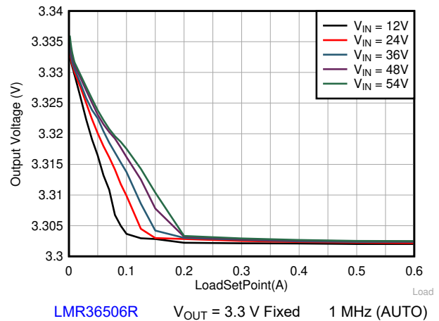
Figure 9-5. Line and Load Regulation
