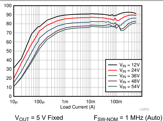
Figure 7-4. Efficiency 5-V Output, Auto Mode
