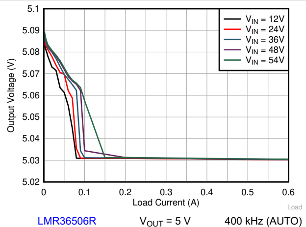
Figure 9-7. Line and Load Regulation
