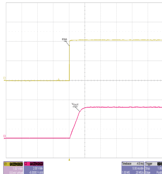
Figure 23. TPS54233-Q1 Start-up Relative to Enable
