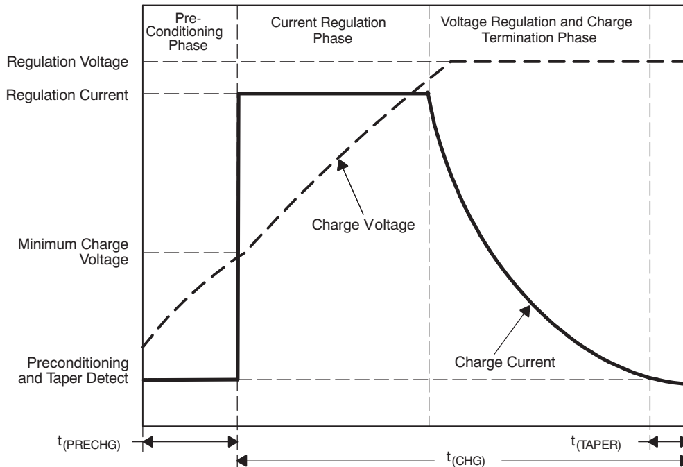
Figure 26. Typical Charging Profile
