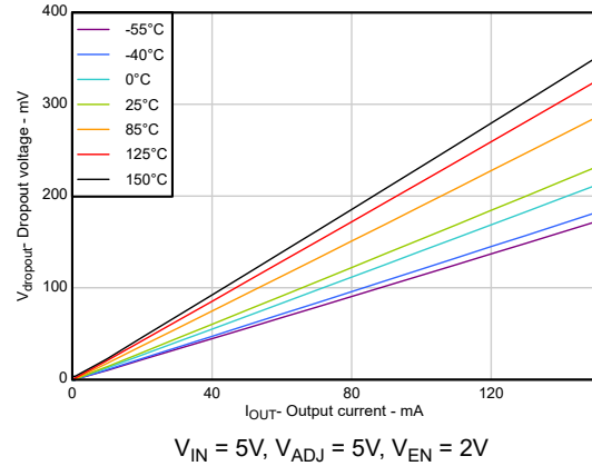
Figure 5-8. Dropout Voltage vs Load Current
