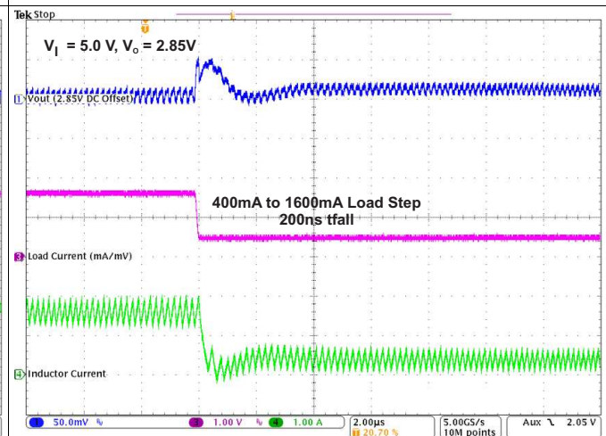
Figure 12. Load Transient Response
