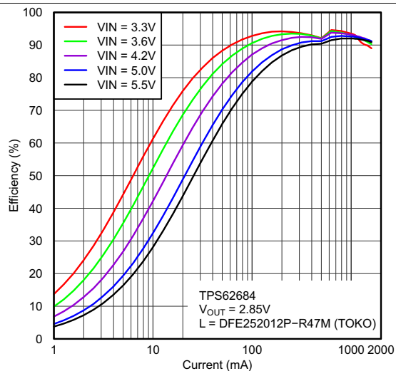
Figure 1. Efficiency Vs Load Current
