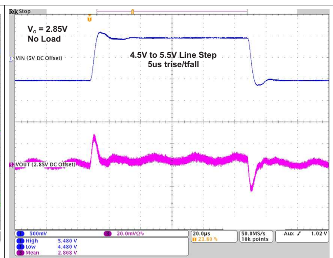
Figure 28. Line Transient Response
