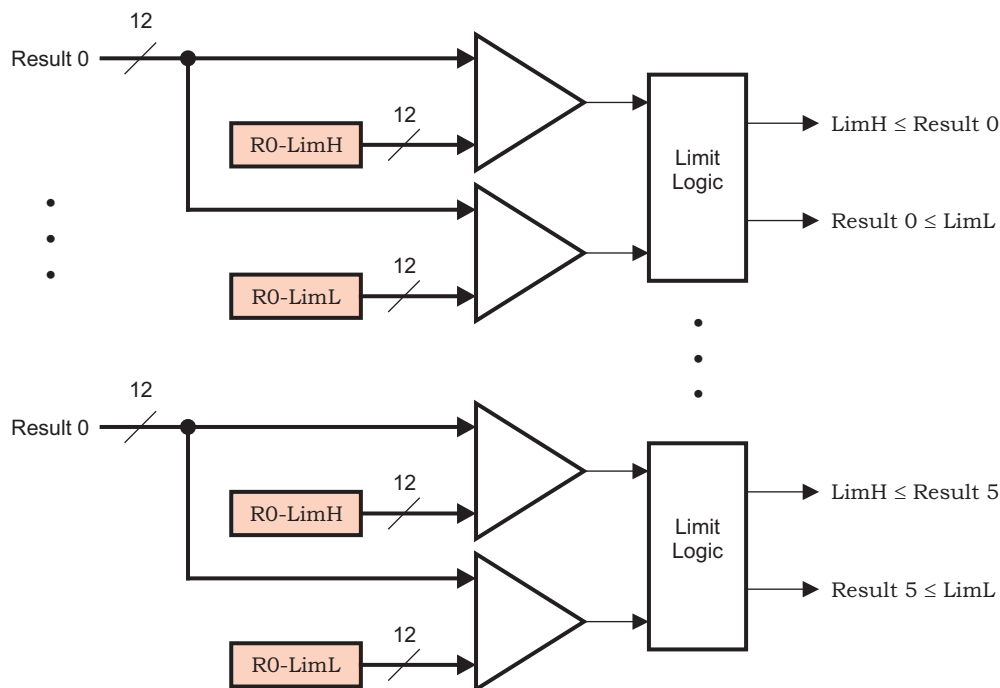
Figure 20. Digital Comparators
