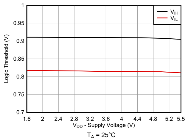
Figure 5-9. Logic Threshold vs Supply Voltage
