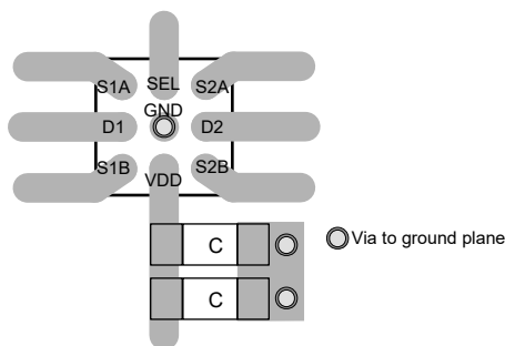
Figure 8-4. TMUX4827 Layout Example
