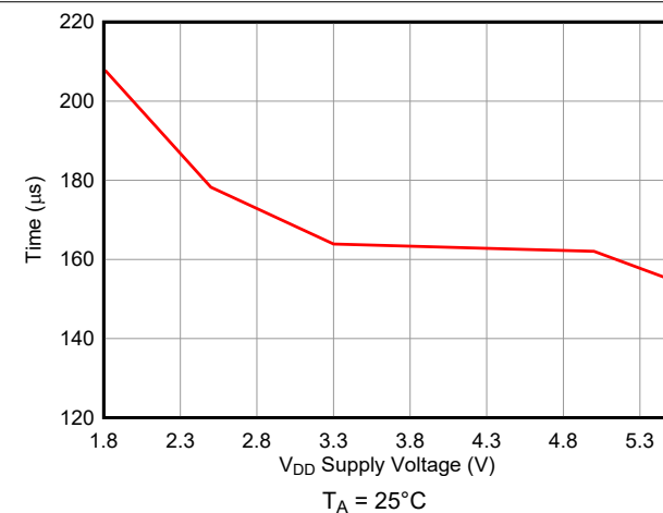
Figure 5-12. tBBM vs Supply Voltage
