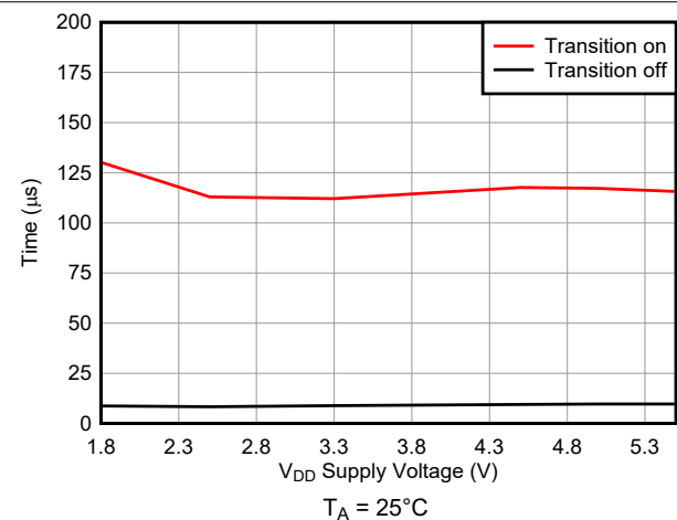
Figure 5-11. Transition Time vs Supply Voltage
