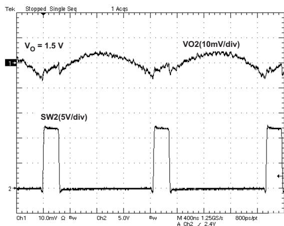
Figure 21. \text{VO2}=1.5\text{ V} , Ripple Voltage ( I_{O2}=3\text{ A} )
