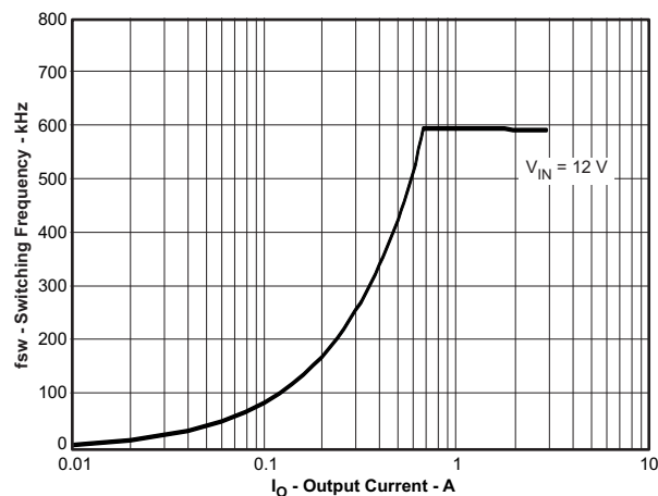
Figure 19. \text{VO2}=1.5\text{ V} , SW-frequency vs Output Current
