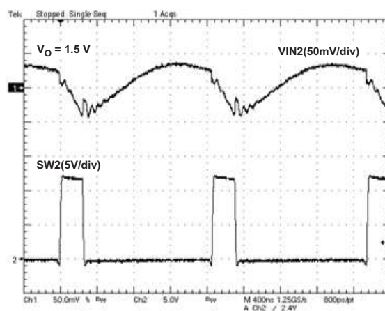
Figure 23. \text{VIN2} Input Voltage Ripple ( I_{O2}=3\text{ A} )
