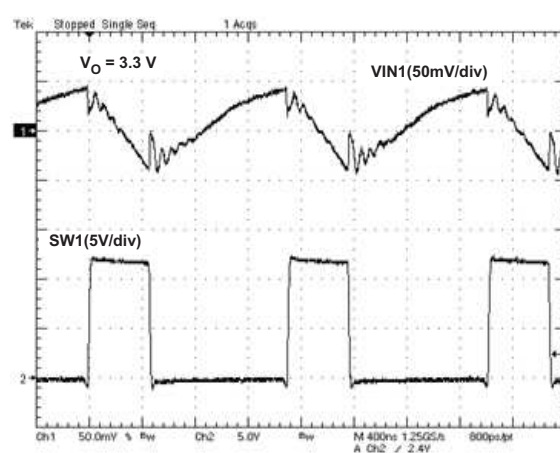
Figure 22. \text{VIN1} Input Voltage Ripple ( I_{O1}=3\text{ A} )
