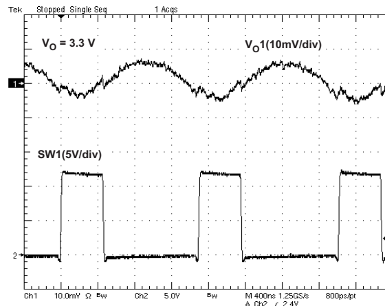
Figure 20. \text{VO1}=3.3\text{ V} , \text{VO1} Ripple Voltage ( I_{O1}=3\text{ A} )
