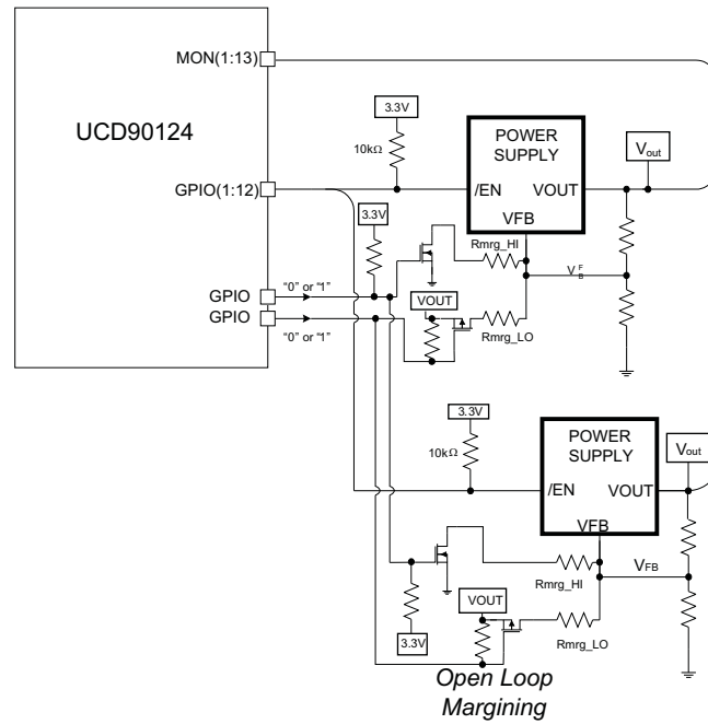
Figure 17. Open-Loop Margining
