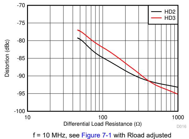
Figure 6-16. Harmonic Distortion vs Rload
