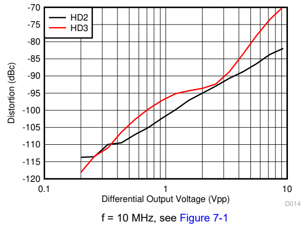
Figure 6-14. Harmonic Distortion vs Output Swing
