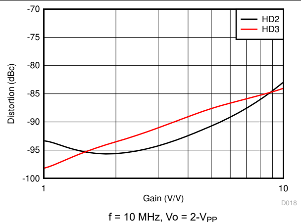
Figure 6-18. Harmonic Distortion vs Gain
