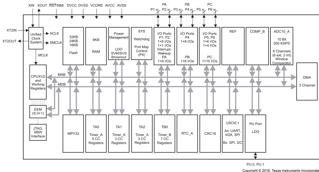
Figure 1-2. Functional Block Diagram – RGZ or PT Package – MSP430F5310, MSP430F5309, MSP430F5308
