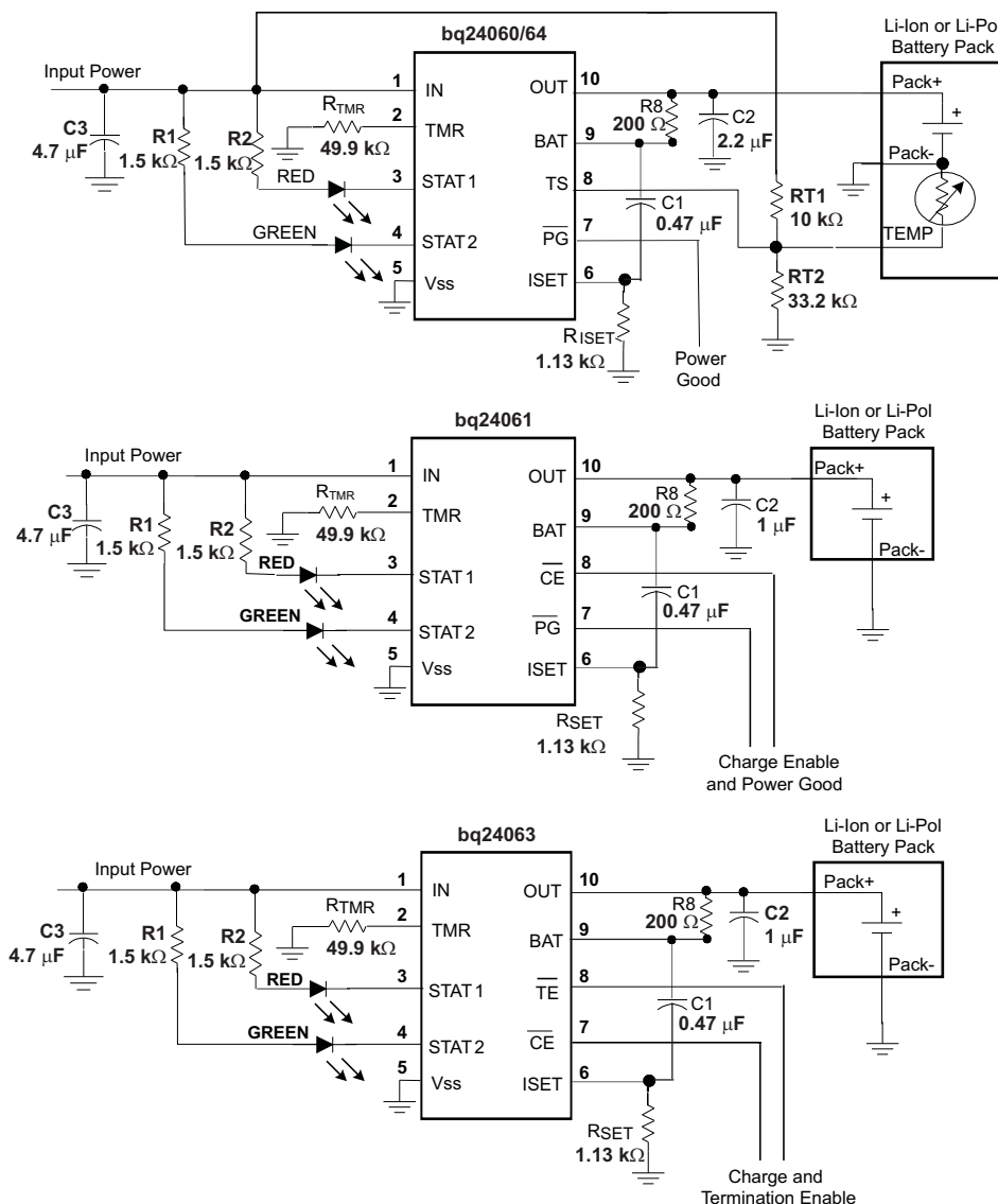
Figure 16. Application Circuits
