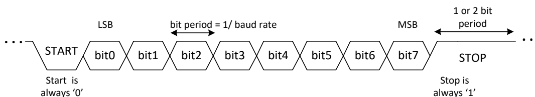
Figure 7-10. UART Character Definition
