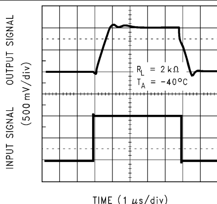
Figure 5-27. Non-Inverting Large Signal Response
