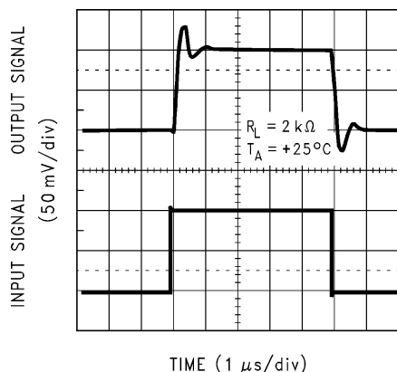
Figure 5-29. Non-Inverting Small Signal Response
