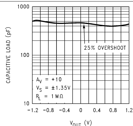
Figure 5-42. Stability vs Capacitive Load
