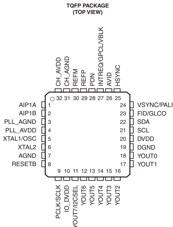
Figure 2-2. Terminal Diagrams
