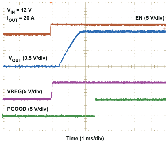
Figure 6-13. Start-Up Waveforms
