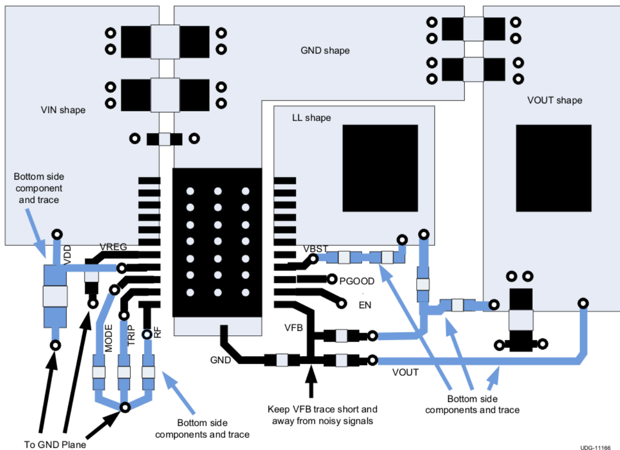
Figure 10-1. Layout Recommendation
