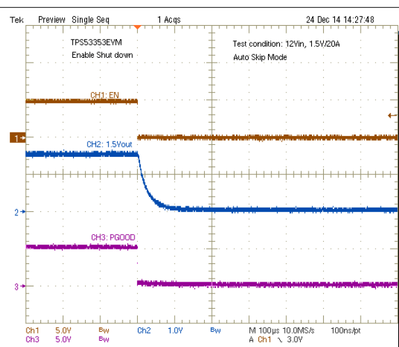
Figure 8-3. Enable Turnoff
