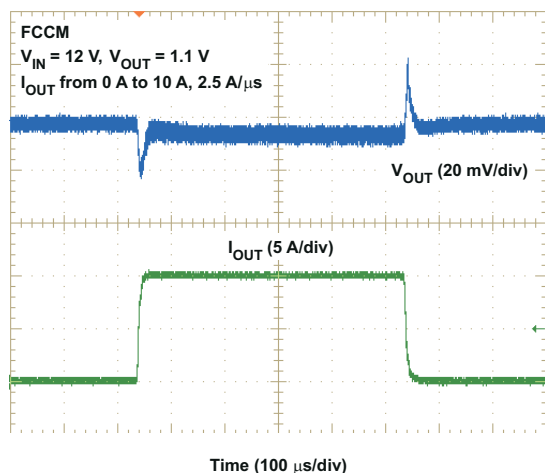
Figure 6-21. FCCM Load Transient
