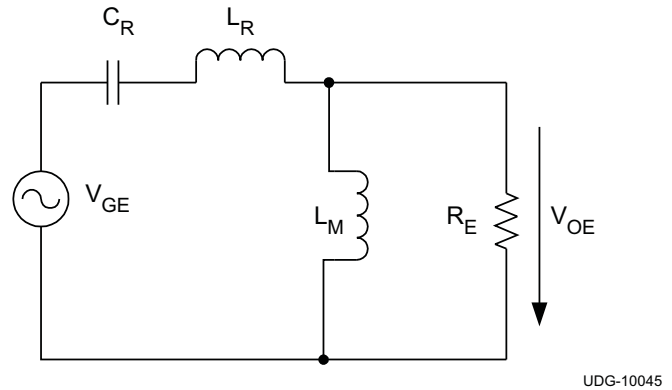
Figure 13. LLC Resonant Converter Equivalent Circuit
