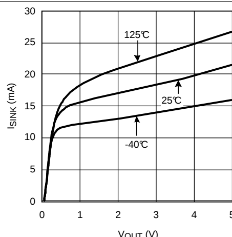
Figure 18. Sinking Current vs Output Voltage
