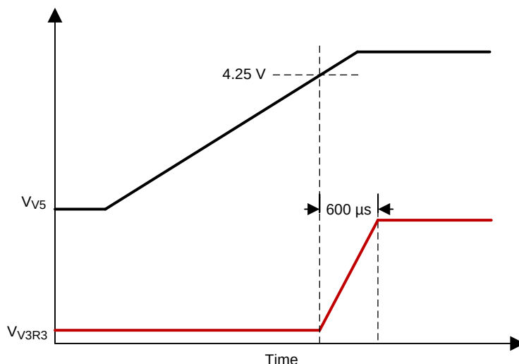
Figure 7. V3R3 Startup Waveform
