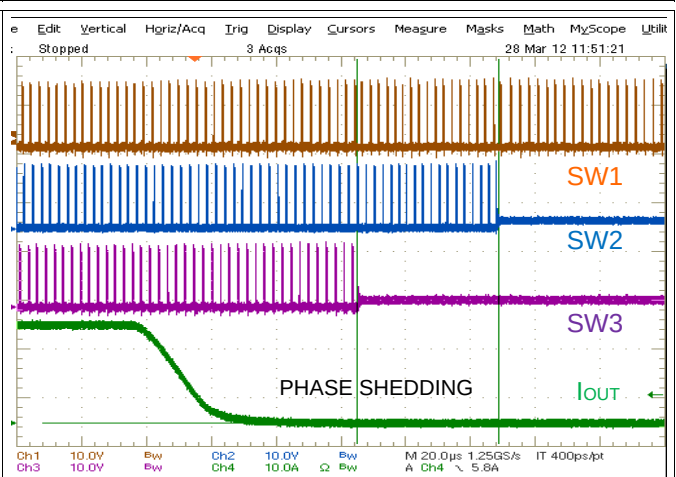
Figure 116. Phase Shedding
