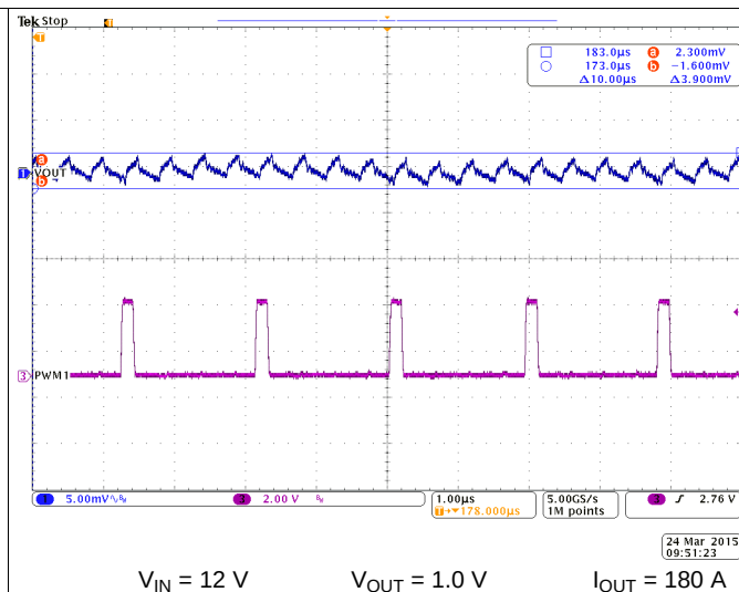
Figure 108. Output Ripple
