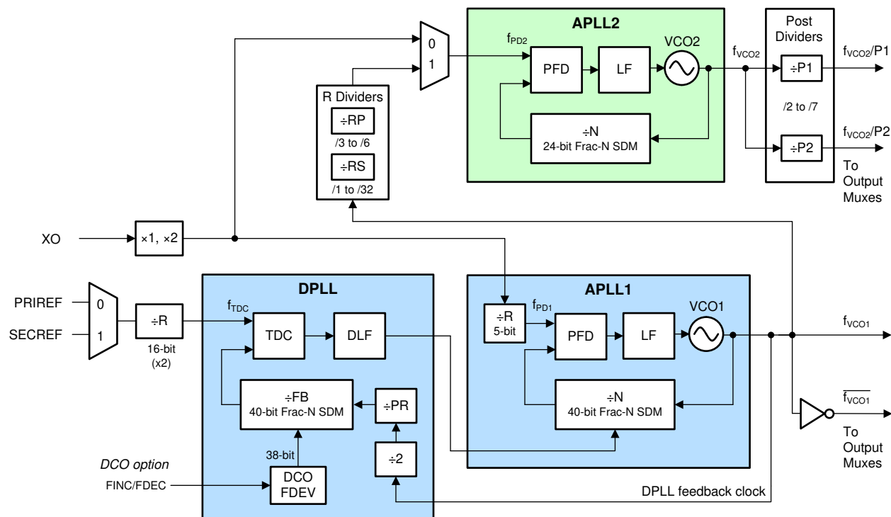
Figure 9-22. PLL Architecture
