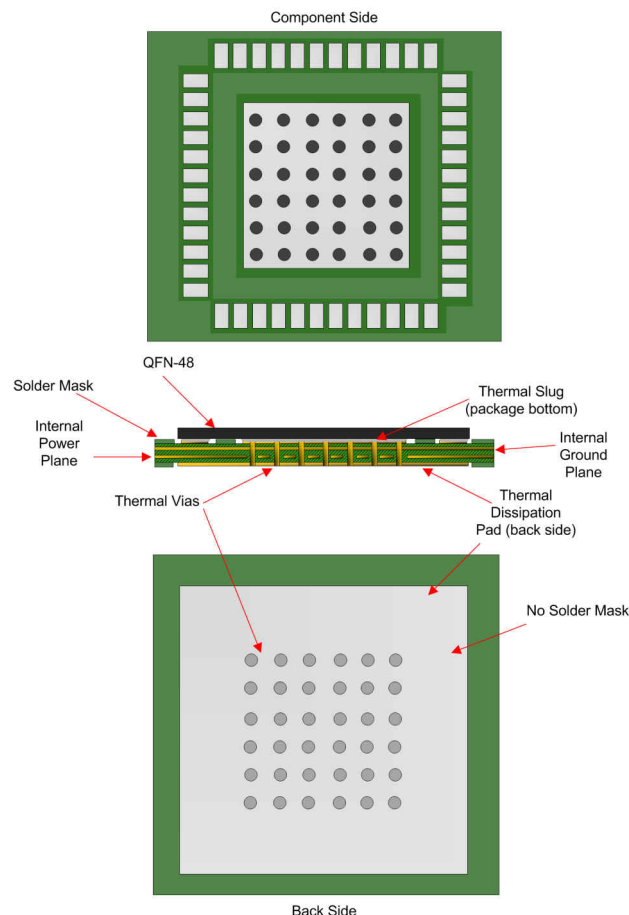
Figure 12-1. General PCB Ground Layout for Thermal Reliability (8+ Layers Recommended)
