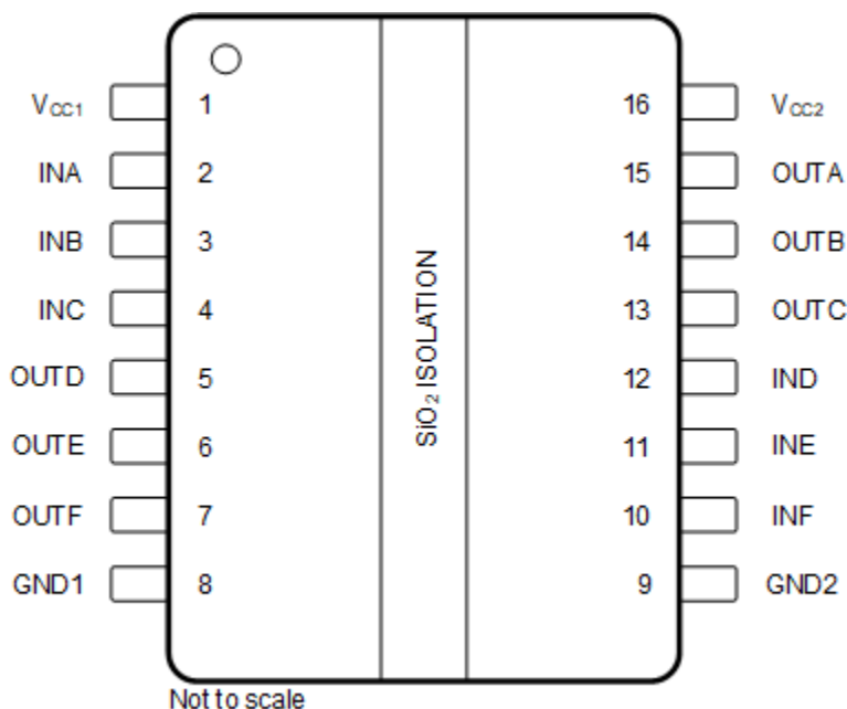
Figure 4-1. DW Package, 16-Pin Wide-SOIC (Top View)
