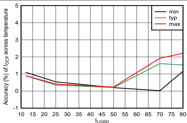
Figure 6-14. I_{OCP} Accuracy vs Load Current
