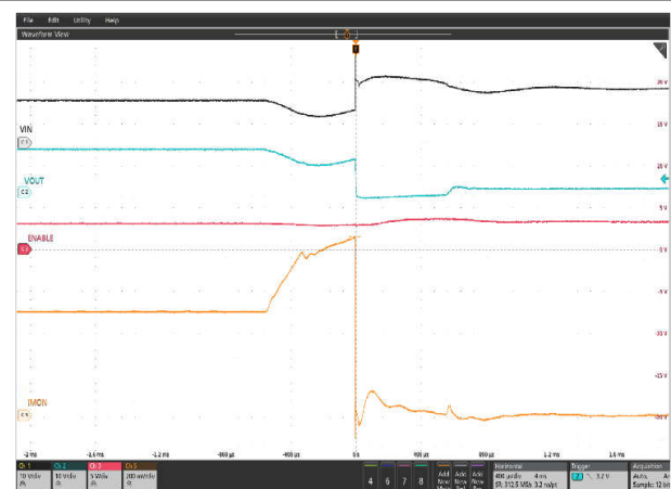
Figure 8-8. Circuit-Breaker Response: V_{IN} = 12\text{V} , C_{LOAD} = 40\text{mF} , R_{IMON} = 167\Omega , R_{REF} = 27\text{k}\Omega , and Load Current Stepped up From 250A to 510A
