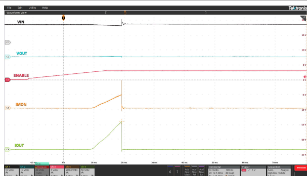
Figure 8-7. Power Up into Short: V_{IN} = 12\text{V} , EN/UVLO Stepped Up From 0V to 3V, R_{REF} = 27\text{k}\Omega , R_{ILIM} on Each Device = 2\text{k}\Omega , and OUT Shorted to GND
