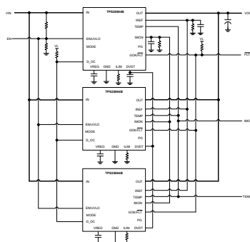
Simplified Schematic
