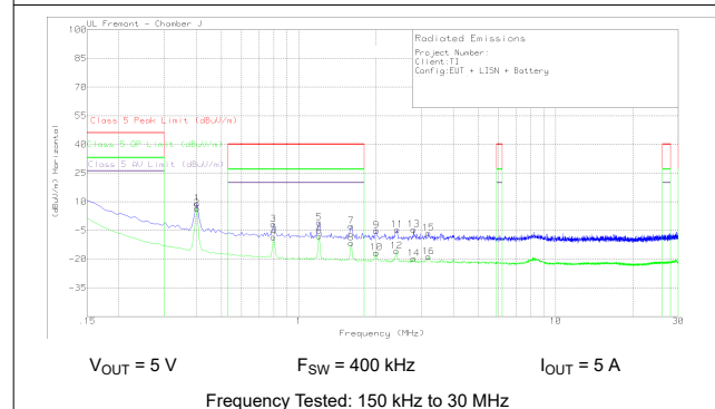
Figure 9-27. Radiated EMI Rod versus CISPR25 Limits
