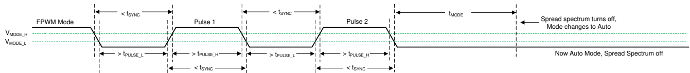
Figure 8-8. Spread Spectrum Disabled in Transition from FPWM Mode to Auto Mode
