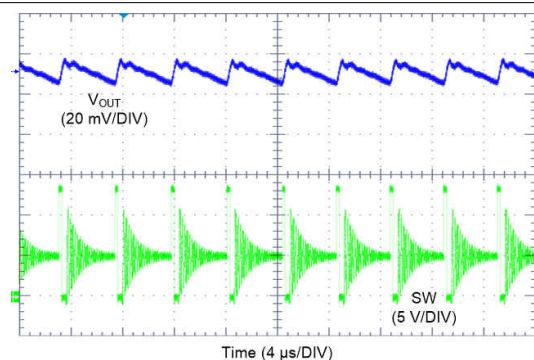
Figure 9-17. LM62435-Q1 Switching Waveform and V_{OUT} Ripple
