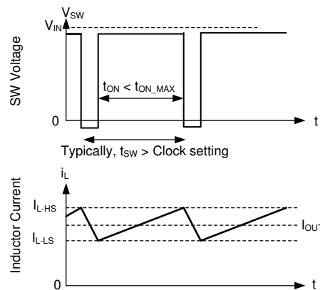
Figure 8-18. Current Limit Waveforms
