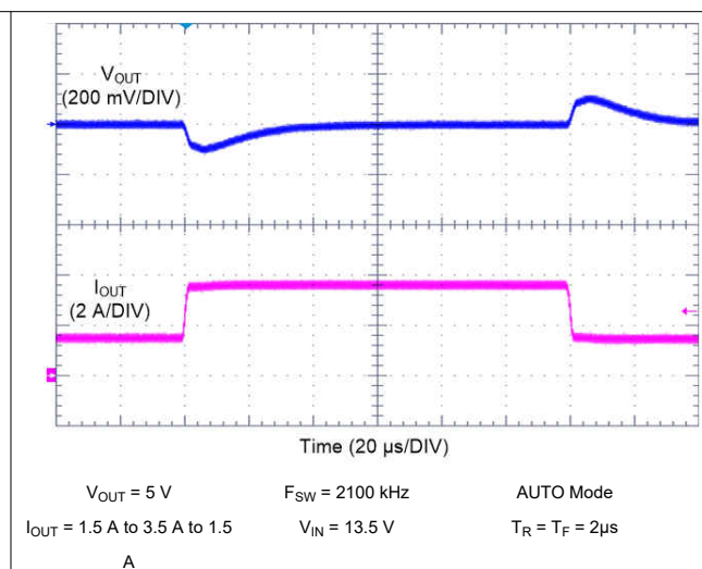
Figure 9-24. LM62435-Q1 Load Transient
