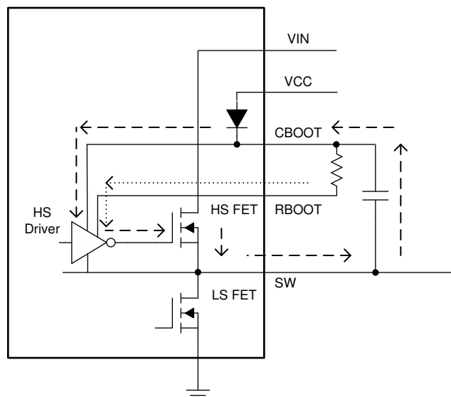
Figure 8-14. Simplified Circuit Showing How RBOOT Functions
