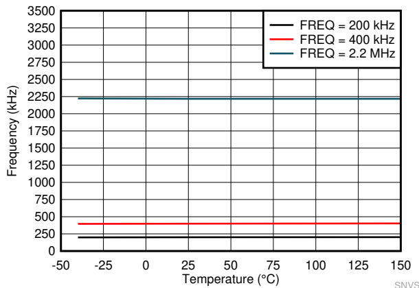
Figure 7-5. Switching Frequency Set by SYNC
