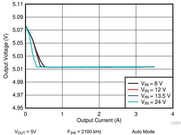
Figure 9-11. LM62435-Q1 Load and Line Regulation
