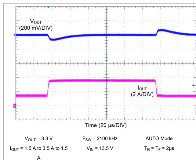
Figure 9-23. LM62435-Q1 Load Transient
