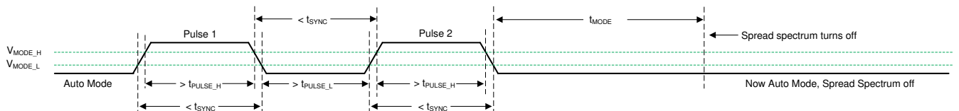
Figure 8-7. Spread Spectrum Disabled in Auto Mode
