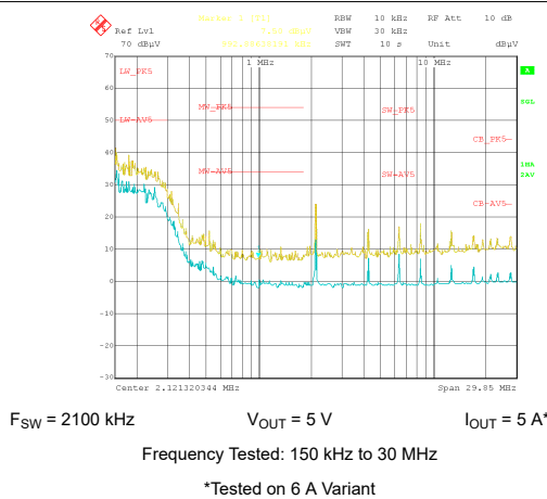
Figure 9-33. Conducted EMI versus CISPR25 Limits (Yellow: Peak Signal, Blue: Average Signal)
