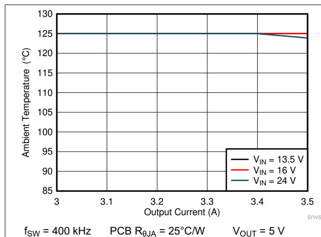
Figure 9-2. Maximum Ambient Temperature versus Output Current
