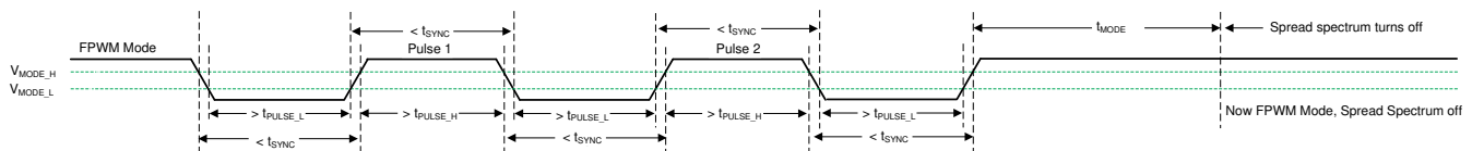
Figure 8-6. Spread Spectrum Disabled in FPWM Mode
