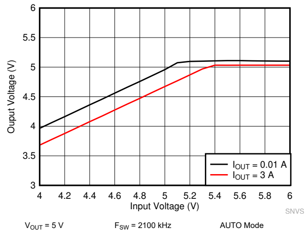
Figure 9-14. LM62435-Q1 Dropout Curve
