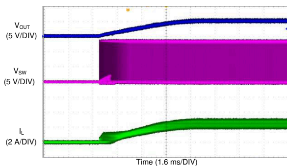
Figure 9-19. LM62435-Q1 Start-up with 3.25 A
