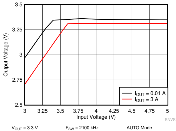
Figure 9-13. LM62435-Q1 Dropout Curve
