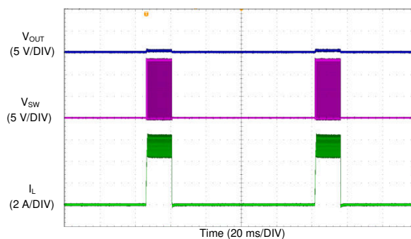
Figure 9-20. LM62435-Q1 Short Circuit Protection
