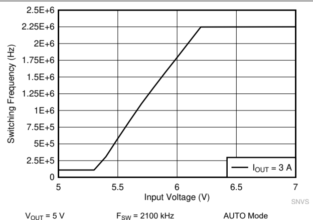
Figure 9-16. LM62435-Q1 Frequency Dropout Curve
