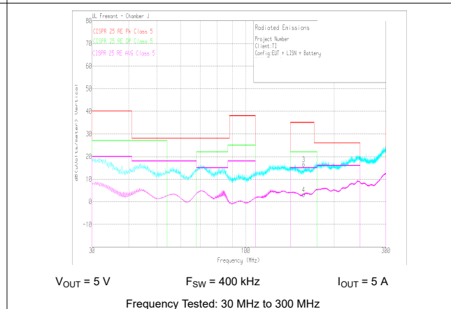
Figure 9-28. Radiated EMI Bicon Vertical versus CISPR25 Limits
