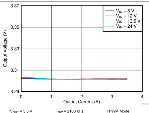
Figure 9-10. LM62435-Q1 Load and Line Regulation
