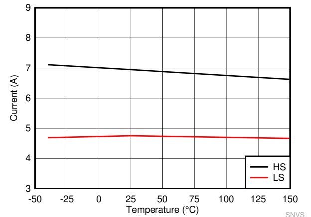
Figure 7-4. LM62435-Q1 High-side and Low-side Current Limits
