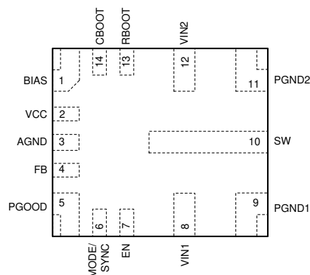
Figure 6-1. RJR Package 14-Pin VQFN-HR Top View
