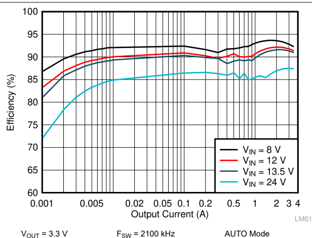
Figure 9-5. LM62435-Q1 Efficiency
