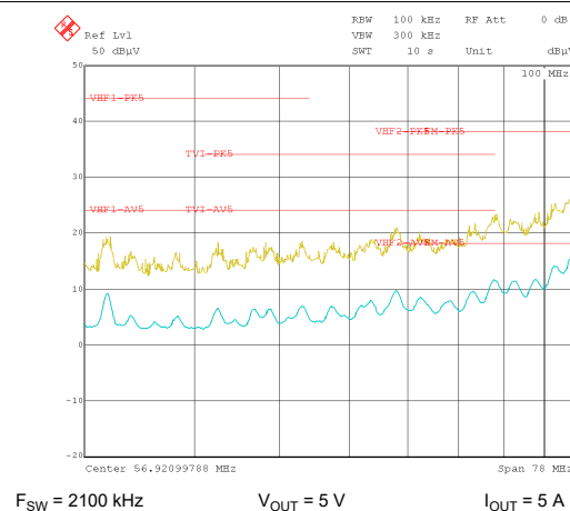
Figure 9-34. Conducted EMI versus CISPR25 Limits (Yellow: Peak Signal, Blue: Average Signal)
