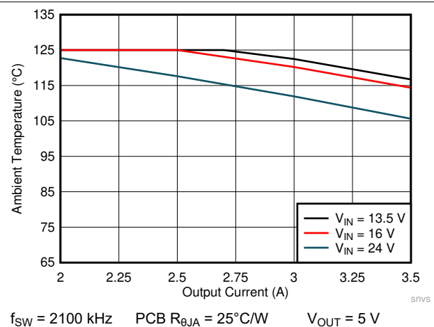
Figure 9-3. Maximum Ambient Temperature versus Output Current
