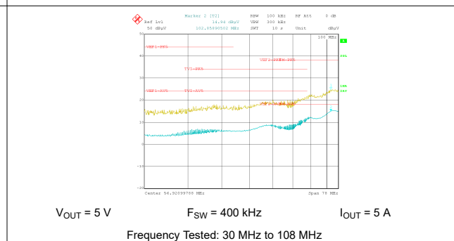
Figure 9-26. Conducted EMI versus CISPR25 Limits (Yellow: Peak Signal, Blue: Average Signal)
