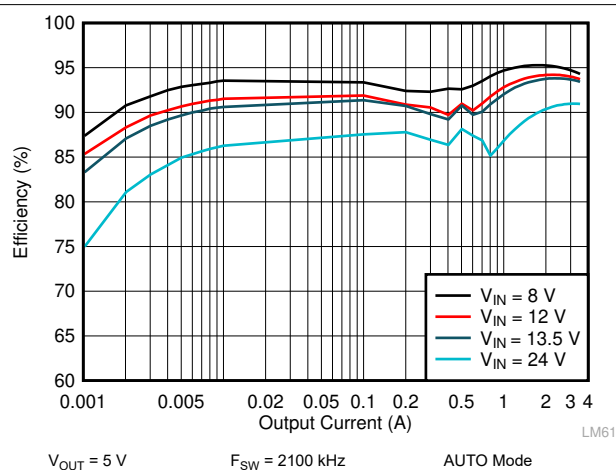
Figure 9-7. LM62435-Q1 Efficiency
