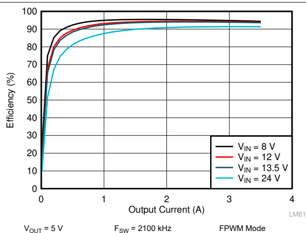
Figure 9-8. LM62435-Q1 Efficiency
