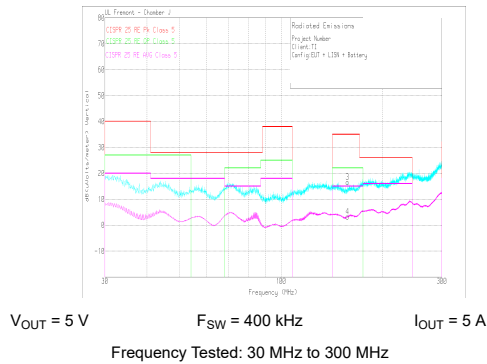
Figure 9-29. Radiated EMI Bicon Horizontal versus CISPR25 Limits
