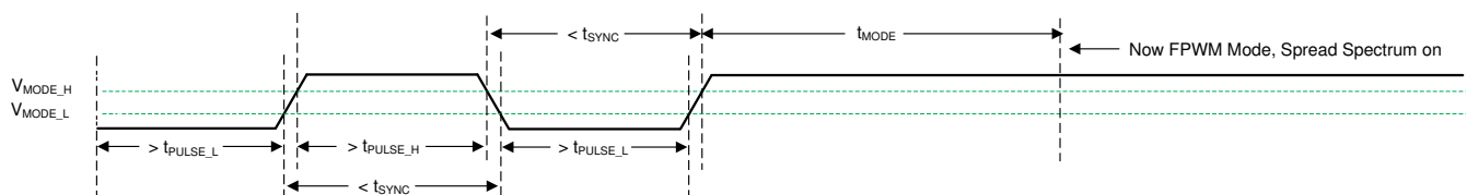
Figure 8-11. Transition from SYNC Mode to FPWM Mode
