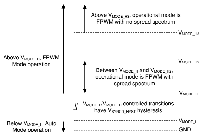
Figure 8-2. Level-Dependent Mode Selection Settings
