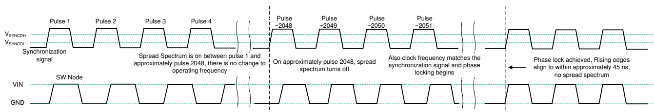
Figure 8-12. Synchronization Process
