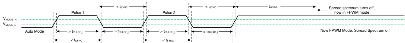
Figure 8-9. Spread Spectrum Disabled in Transition from Auto Mode to FPWM Mode
