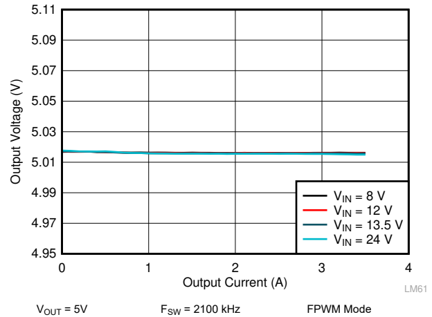
Figure 9-12. LM62435-Q1 Load and Line Regulation
