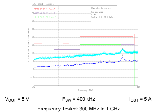
Figure 9-30. Radiated EMI Log Vertical versus CISPR25 Limits
