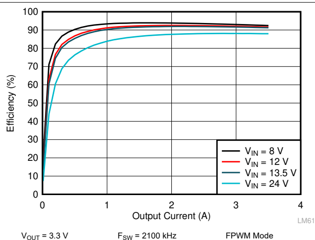
Figure 9-6. LM62435-Q1 Efficiency
