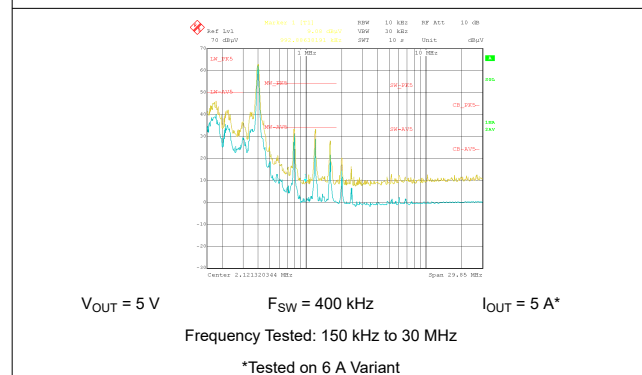
Figure 9-25. Conducted EMI versus CISPR25 Limits (Yellow: Peak Signal, Blue: Average Signal)
