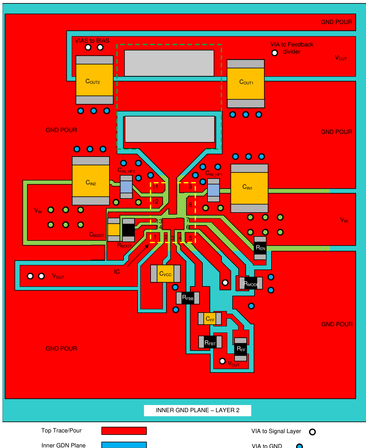
Figure 11-2. Layout Example
