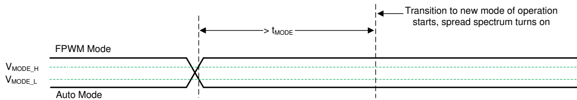
Figure 8-5. Transition from Auto Mode and FPWM Mode
