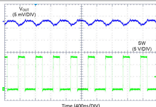
Figure 9-18. LM62435-Q1 Switching Waveform and V_{OUT} Ripple
