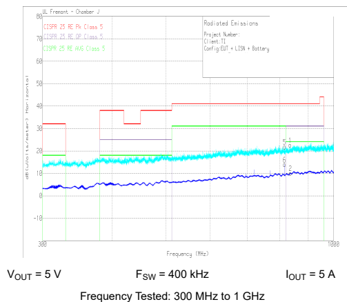
Figure 9-31. Radiated EMI Log Horizontal versus CISPR25 Limits
