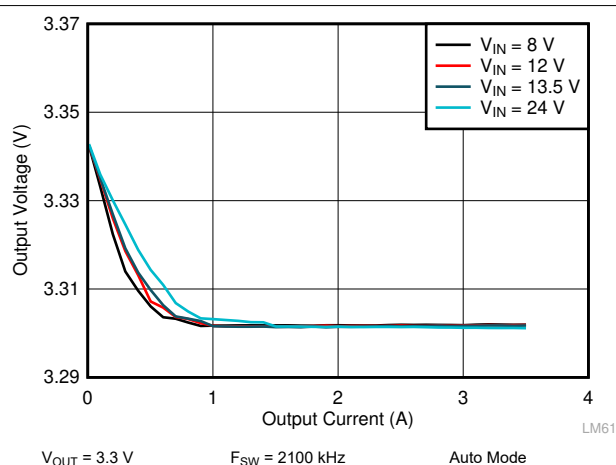
Figure 9-9. LM62435-Q1 Load and Line Regulation
