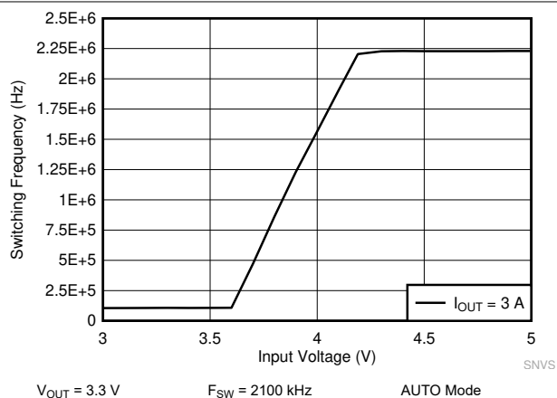
Figure 9-15. LM62435-Q1 Frequency Dropout Curve
