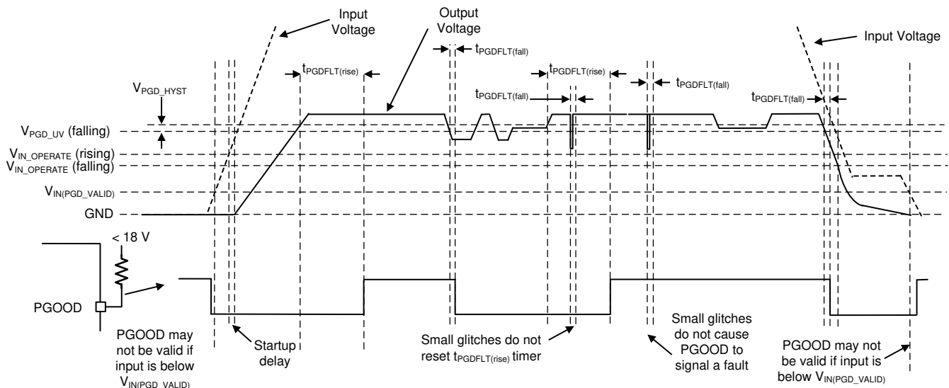
Figure 8-13. PGOOD Timing Diagram (Excludes OV Events)
