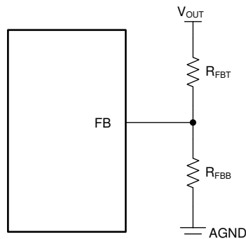
Figure 8-17. Setting Output Voltage of Adjustable Versions
