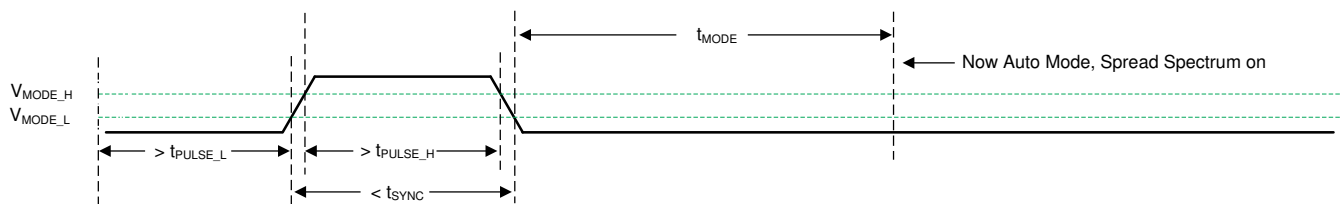
Figure 8-10. Transition from SYNC Mode to Auto Mode
