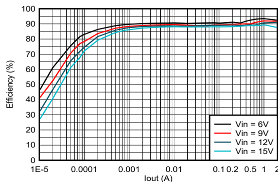
Efficiency Versus Output Current (3.3 V_O at 2.5 MHz, 1 \mu\text{H} , Auto PFM or PWM)
