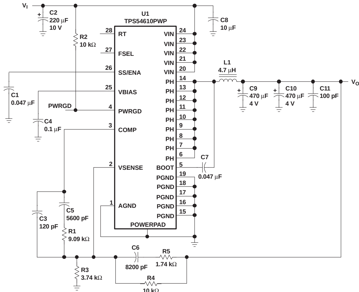
Figure 10. Application Circuit
