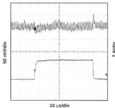
Figure 22. TRANSIENT RESPONSE, 1.5-A to 4.5-A STEP
