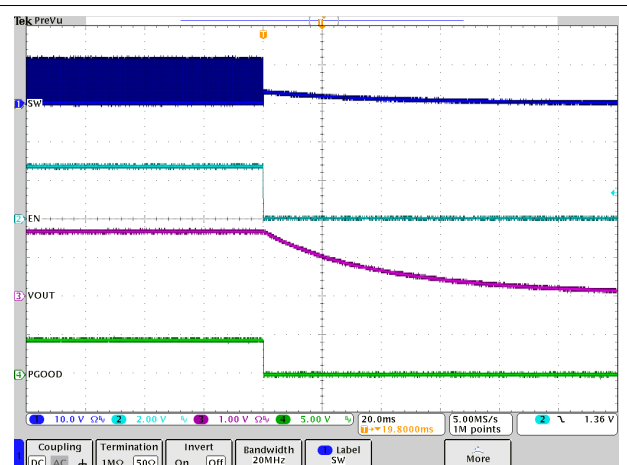
Figure 8-13. ENABLE Shutdown Waveform, PVIN = 12 V, VOUT = 1.8 V
