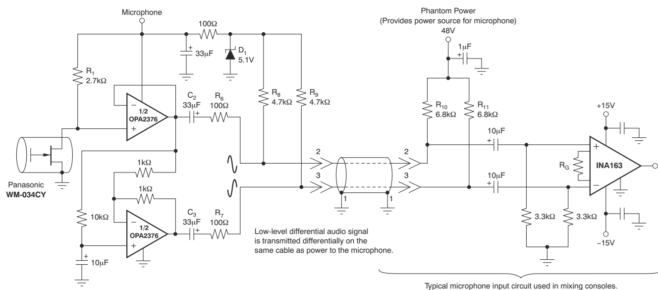
Figure 8-4. Phantom-Powered Electret Microphone
