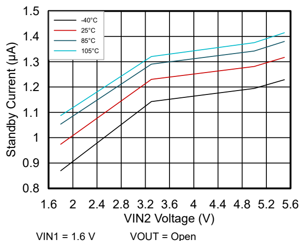
Figure 6-5. VIN2 Standby Current vs Input Voltage
