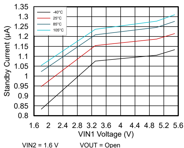
Figure 6-4. VIN1 Standby Current vs Input Voltage
