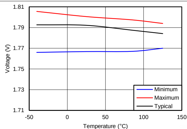
Figure 5-10. BP18 Voltage vs Temperature
