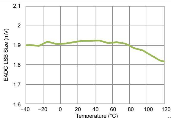
Figure 5-9. EADC LSB Size With 4X Gain (mV) vs Temperature
