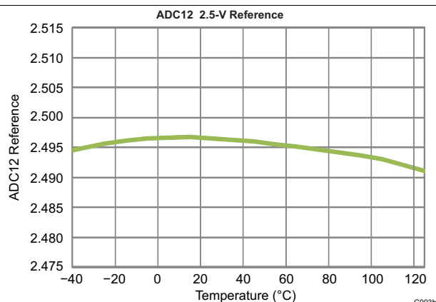
Figure 5-12. ADC12 2.5-V Reference vs Temperature
