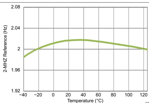
Figure 5-14. Oscillator Frequency (2-MHz Reference, Divided Down from 250 MHz) vs Temperature
