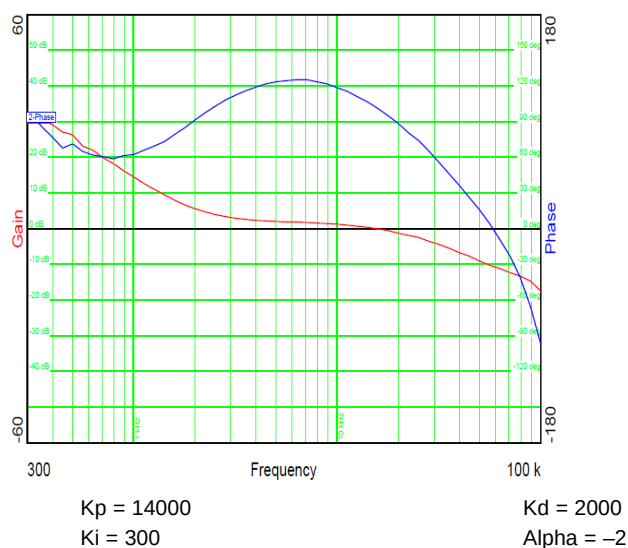
Figure 8-17. Bode Plot
