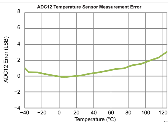
Figure 5-13. ADC12 Temperature Sensor Measurement Error vs Temperature
