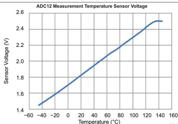
Figure 5-11. ADC12 Measurement Temperature Sensor Voltage vs Temperature
