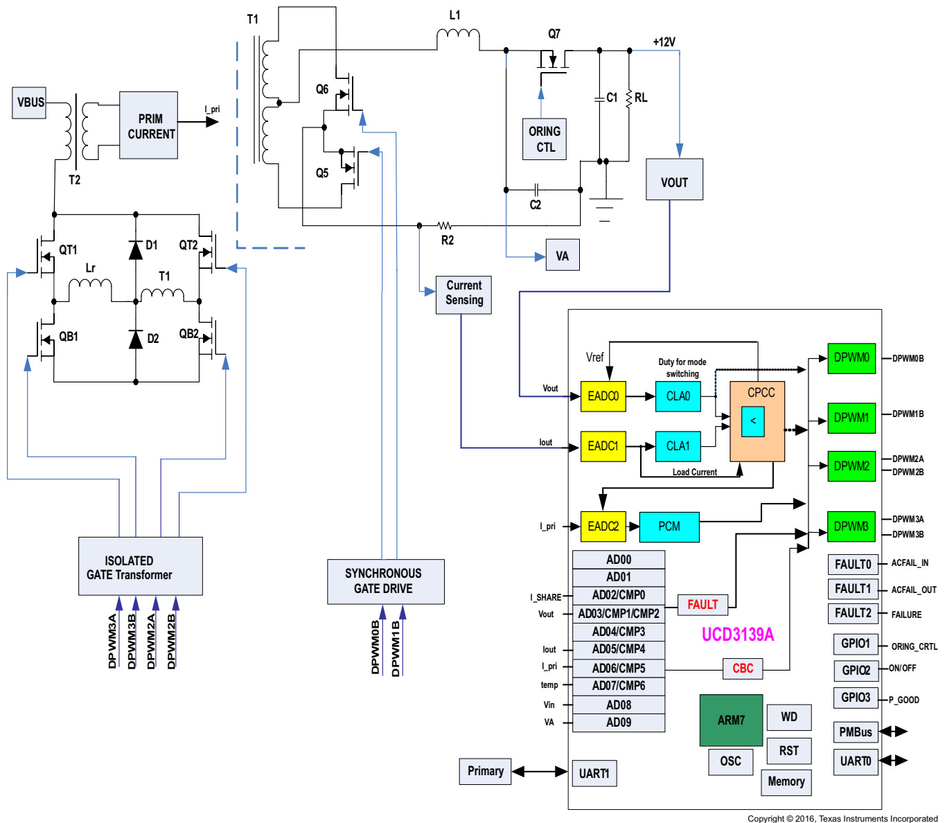
Figure 8-6. Phase-Shifted Full-Bridge Topology
