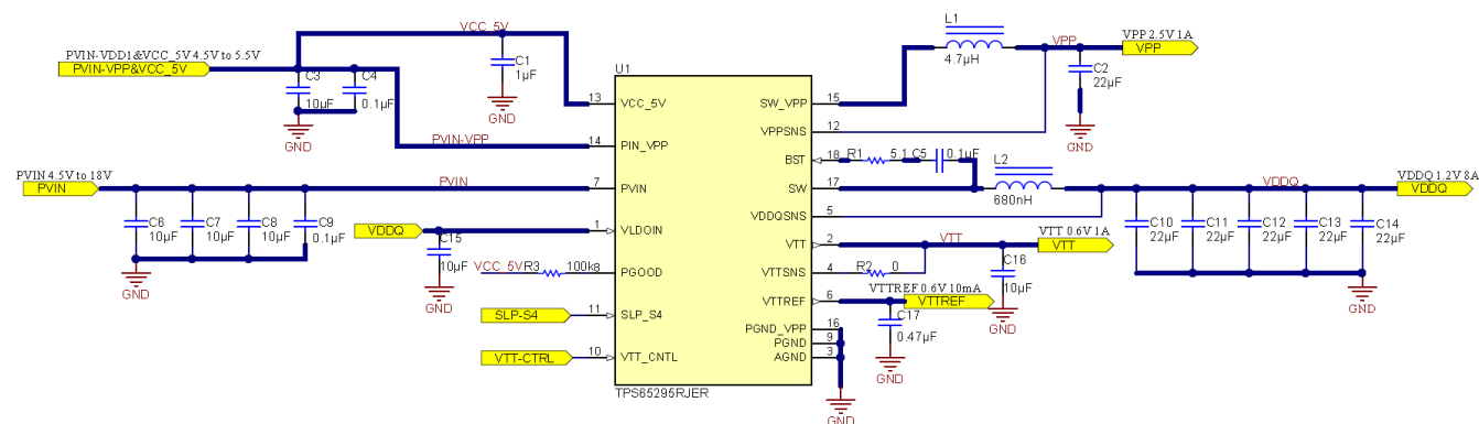
Figure 31. Application Schematic
