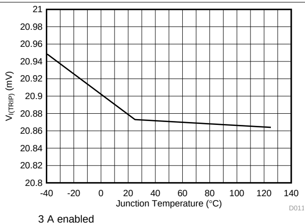
Figure 16. V_{(I(TRIP))} When V_{(VPWR)} > 4.65 V
