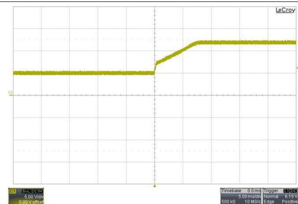
Figure 48. Load Regulation
