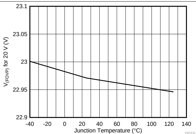
Figure 14. V_{(FOVP)} While Supplying 20 V
