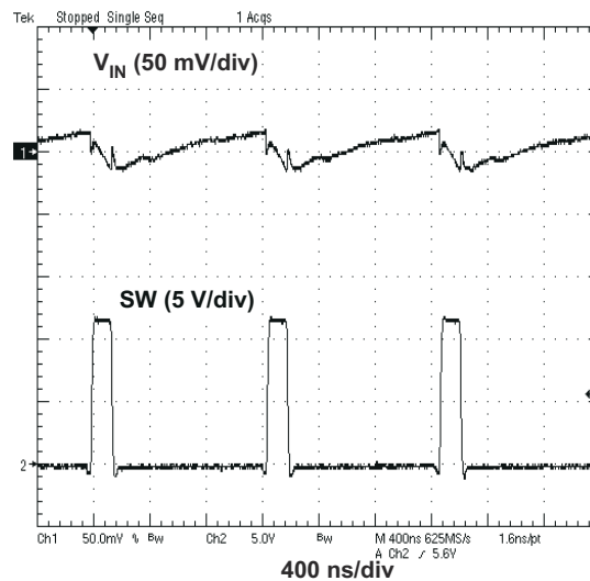
Figure 8-11. Input Voltage Ripple
