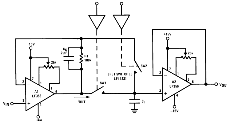
Figure 40. Fast Sample and Hold
