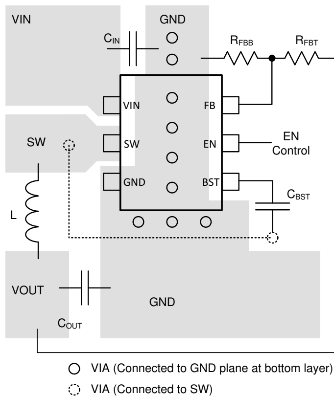
Figure 9-1. TPS562207 Layout
