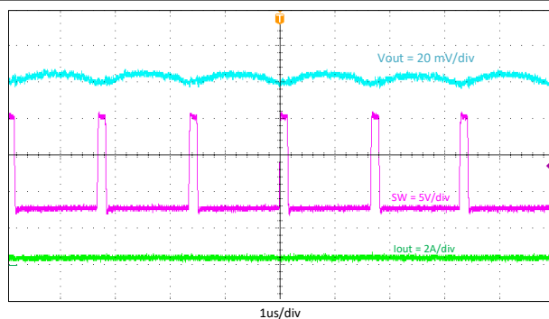
Figure 8-5. Output Voltage Ripple, I_{out} = 0.2 A
