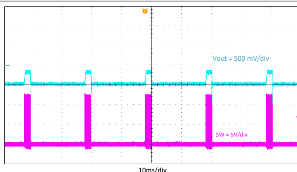
Figure 8-7. Hiccup, I_{out} = 5 A
