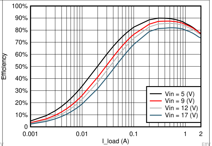
Figure 6-10. V_{OUT} = 1.05 V Efficiency, L = 2.2\mu\text{H}
