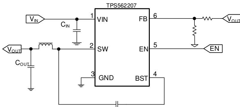
Simplified Schematic
