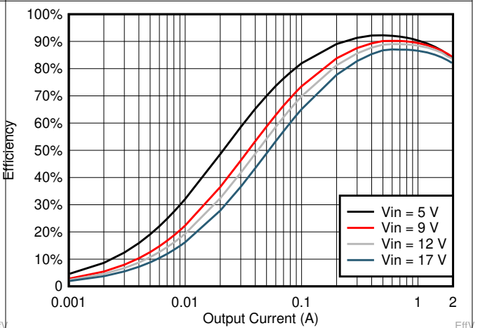
Figure 6-12. V_{OUT} = 1.8 V Efficiency, L = 2.2\mu\text{H}
