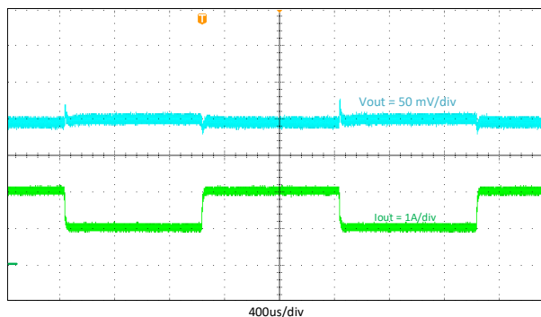
Figure 8-9. Transient Response, 1 to 2 A
