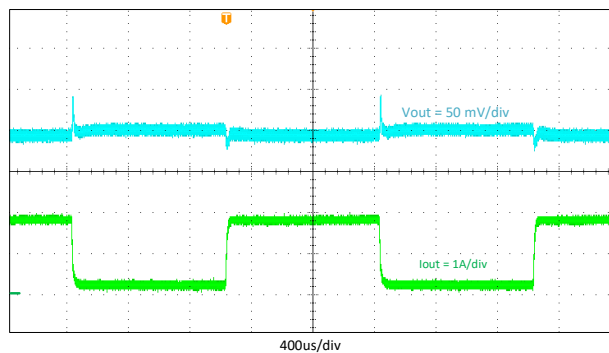
Figure 8-8. Transient Response, 0.2 to 1.8 A
