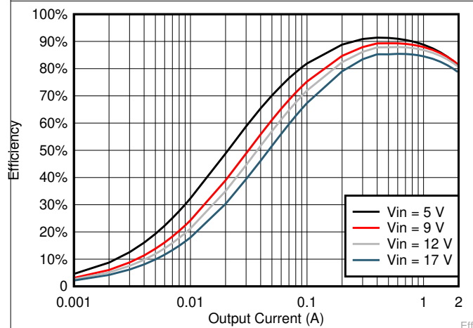
Figure 6-11. V_{OUT} = 1.5 V Efficiency, L = 2.2\mu\text{H}
