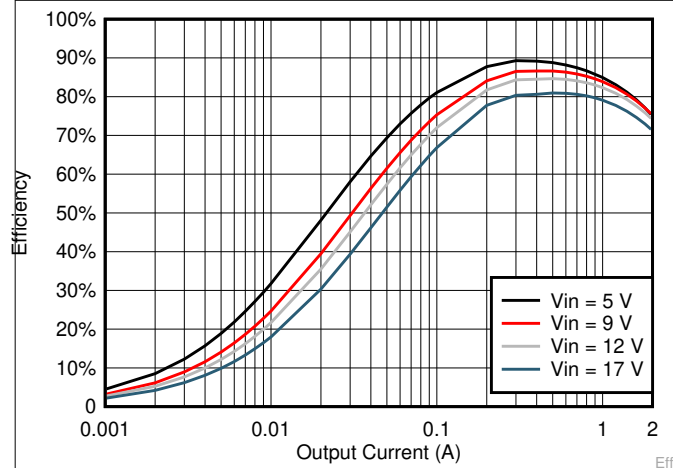
Figure 6-9. V_{OUT} = 0.95 V Efficiency, L = 2.2\mu\text{H}
