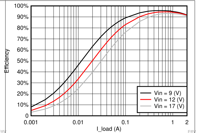
Figure 6-14. V_{OUT} = 5 V Efficiency, L = 4.7 \mu H
