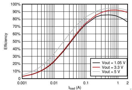
TPS562207 Efficiency
