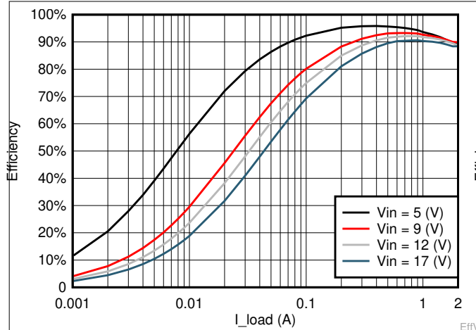
Figure 6-13. V_{OUT} = 3.3 V Efficiency, L = 3.3 \mu H
