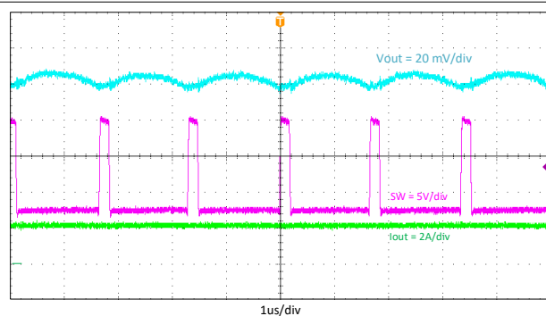
Figure 8-6. Output Voltage Ripple, I_{out} = 2 A
