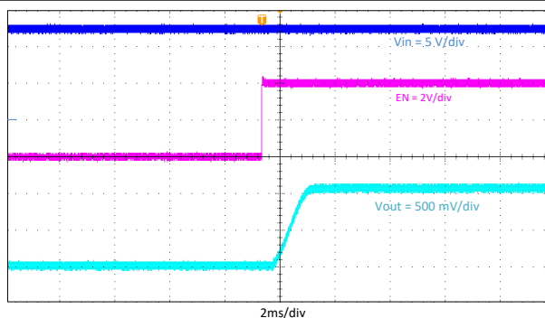
Figure 8-11. Start Up Relative to EN
