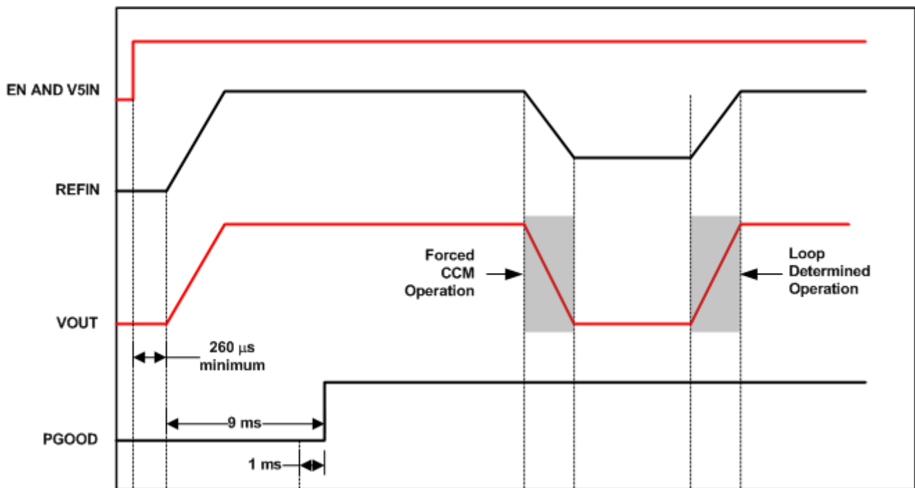
Figure 12. Tracking Start-Up
