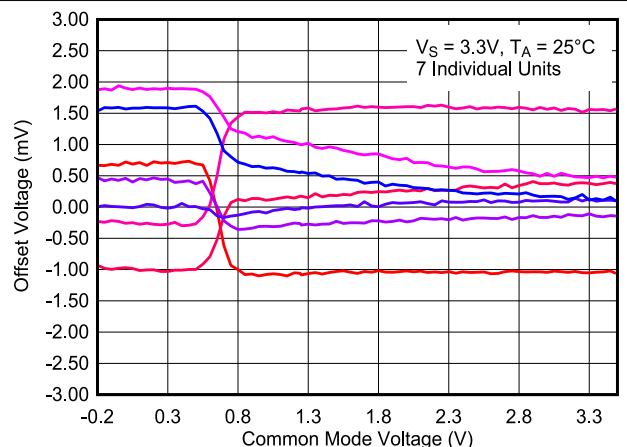
Figure 6-30. Offset Voltage vs. Common Mode Voltage, 3.3V
