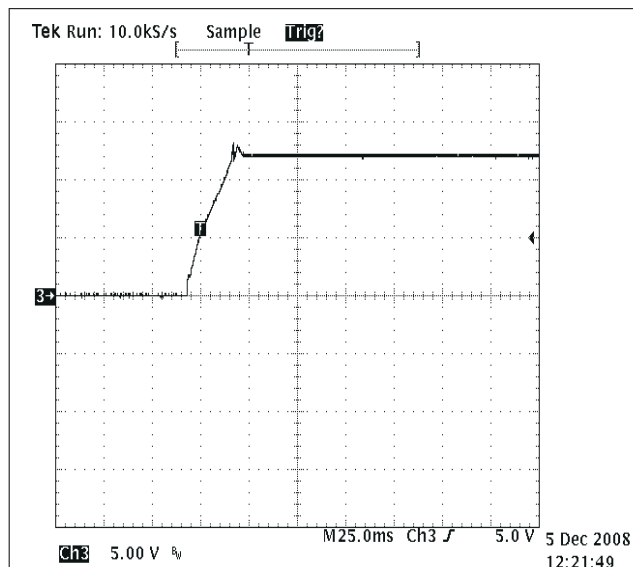
Figure 8-10. Typical Output Voltage Turn On (TP15)
