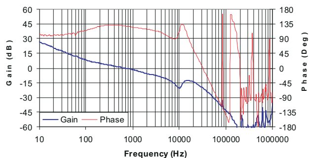
Figure 8-11. Full System Loop Compensation (TP19 and TP21)
