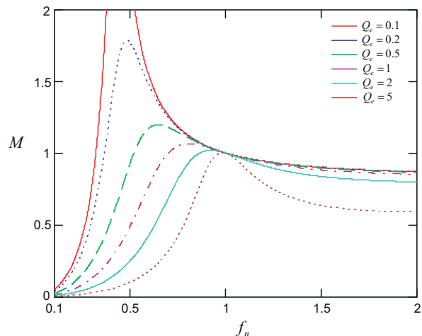
Figure 8-4. M vs f_n
