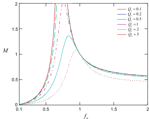
Figure 8-3. M vs f_n
