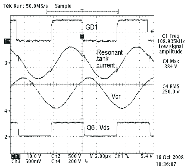
Figure 8-13. Typical Resonant Tank Current and Resonant Capacitor Voltage
