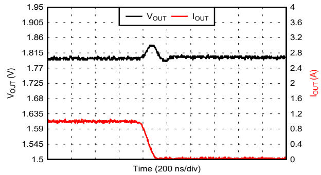
Slew Rate = 8.1 A/ \mu\text{s} I_{OUT} is only the stepped current, parallel 0.5 A load not shown
