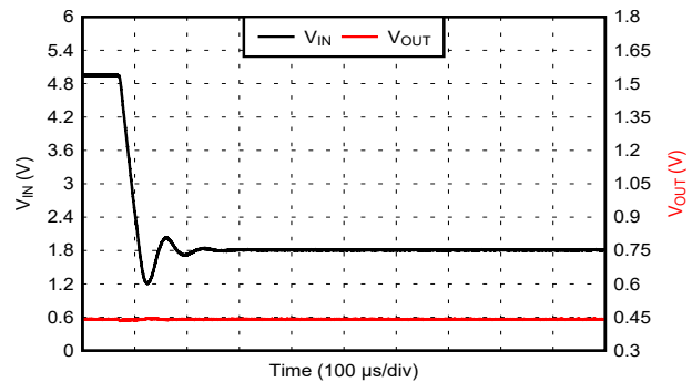
Slew Rate = 85.1 V/ms V_{OUT} = 0.4\text{ V} Figure 6-65. Line Step: 5 V to 1.8 V With I_{OUT} = 1\text{ mA}
