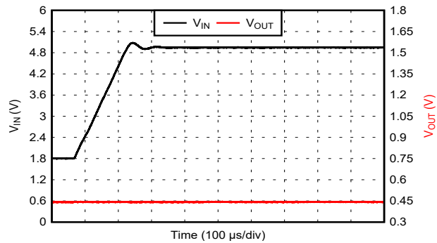
Slew Rate = 20.2 V/ms V_{OUT} = 0.4\text{ V} Figure 6-62. Line Step: 1.8 V to 5 V With I_{OUT} = 1.5\text{ A}
