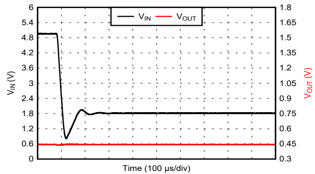
Slew Rate = 144.8 V/ms V_{OUT} = 0.4\text{ V} Figure 6-63. Line Step: 5 V to 1.8 V With I_{OUT} = 1.5\text{ A}
