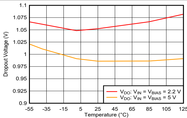
Figure 6-30. Dropout Voltage vs Temperature Without Separate V_{BIAS}
