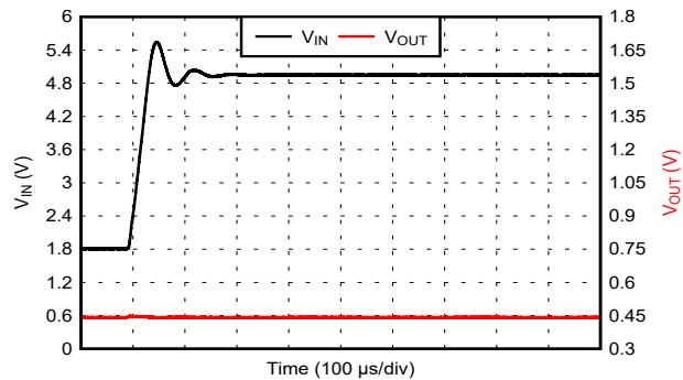
Slew Rate = 84.0 V/ms V_{OUT} = 0.4\text{ V} Figure 6-64. Line Step: 1.8 V to 5 V With I_{OUT} = 1\text{ mA}
