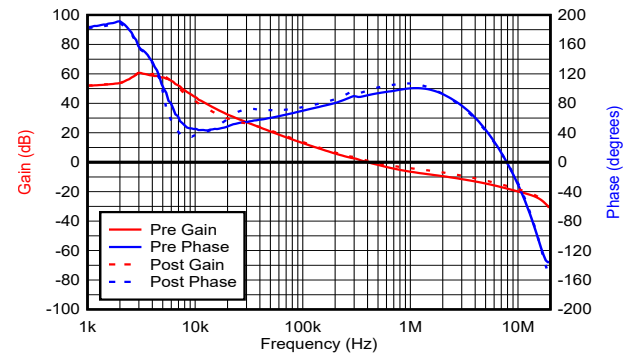
Figure 9-11. Bode Plot: Unit 1 with I_{OUT} = 1 A
