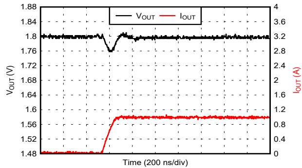
Slew Rate = 8.5 A/ \mu\text{s} I_{OUT} is only the stepped current, parallel 0.5 A load not shown
