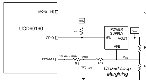
Figure 21. Closed-Loop Margining
