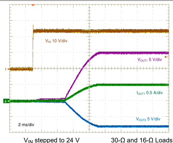
Figure 8-21. Start-Up Characteristic
