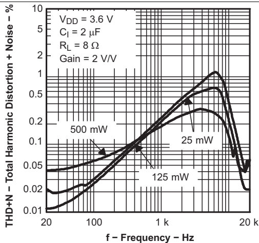
Figure 17. Total Harmonic Distortion + Noise vs Frequency
