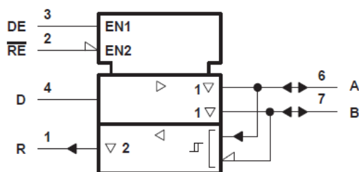
Logic Symbol
