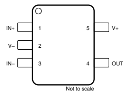
MCP6291 DCK Package 5-Pin SC70 Top View
