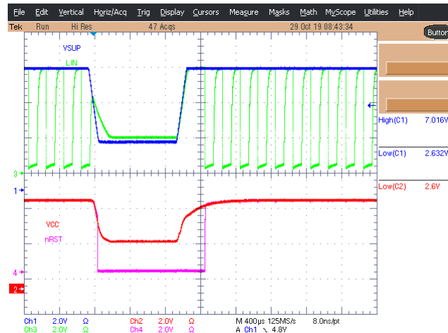
Figure 10-10. TLIN10285S-Q1 Brownout
