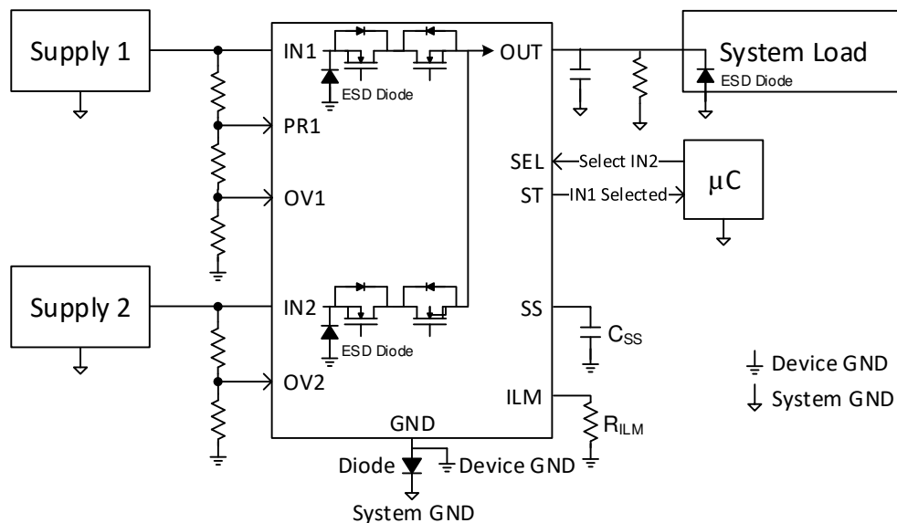
Figure 21. TPS2124 Reverse Polarity Configuration
