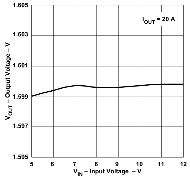
Figure 2. Line Regulation
