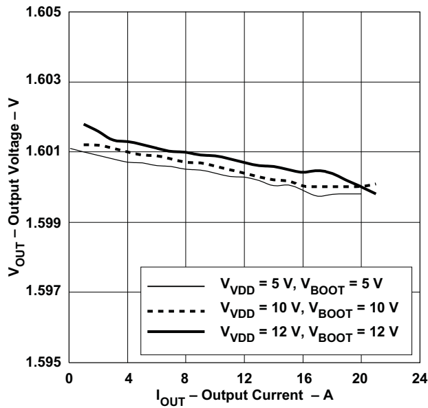
Figure 1. Load Regulation
