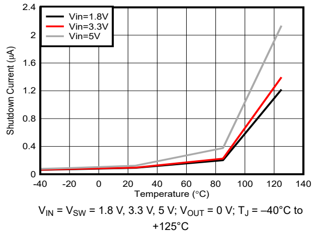
Figure 6-9. Shutdown Current vs Temperature
