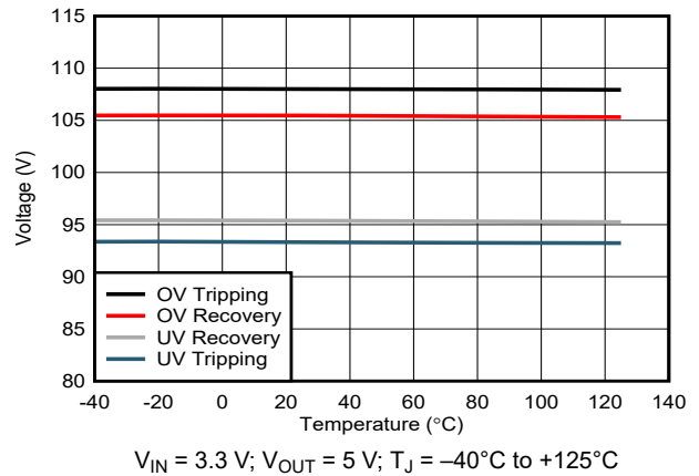
Figure 6-10. PGOOD threshold vs Temperature
