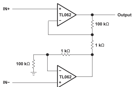
Figure 9-10. Instrumentation Amplifier
