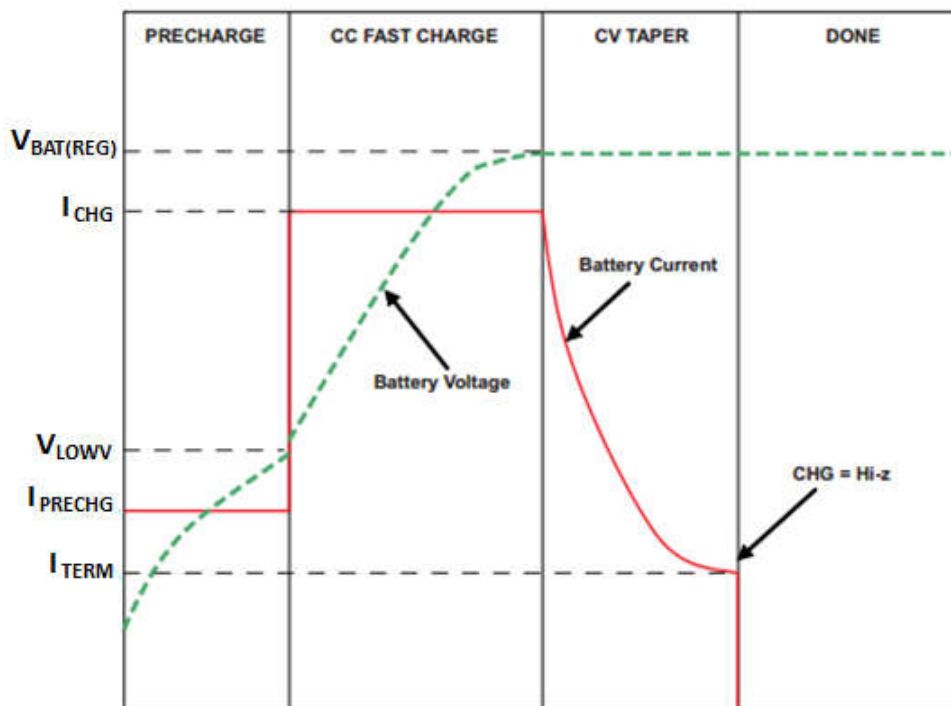
Figure 9-2. BQ25157 Typical Charge Cycle
