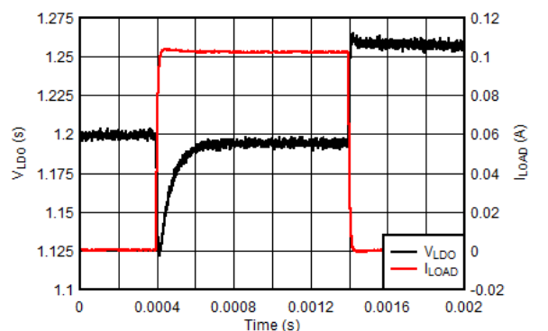
Figure 10-20. LDO Load Transient - VLDO = 1.2V
