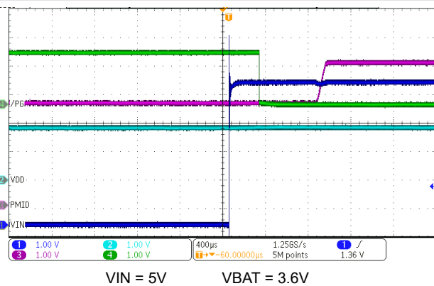
Figure 10-10. \overline{\text{PG}} Power Good Function - IN Supply Insertion
