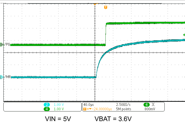
Figure 10-12. \overline{\text{PG}} \overline{\text{MR}} Level Shift Function - \overline{\text{MR}} Rising
